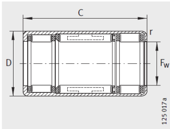
HFL、HFL...KF、滚动轴承布置 ( F_w \geq 8 mm, C \geq 22 mm)、 HFL0822-KF-R、HFL0822-R
