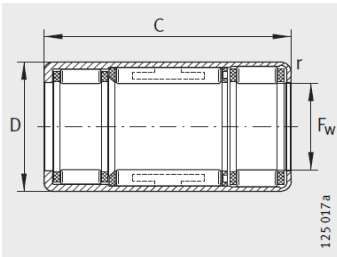
HFL、HFL...KF、滚动轴承布置 ( F_w \geq 8 mm, C \geq 22 mm)、 HFL0822-KF-R、HFL0822-R
