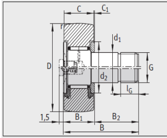
KR16, KR19 KR16-PP, KR19-PP (KRV16-PP, KRV19-PP)
